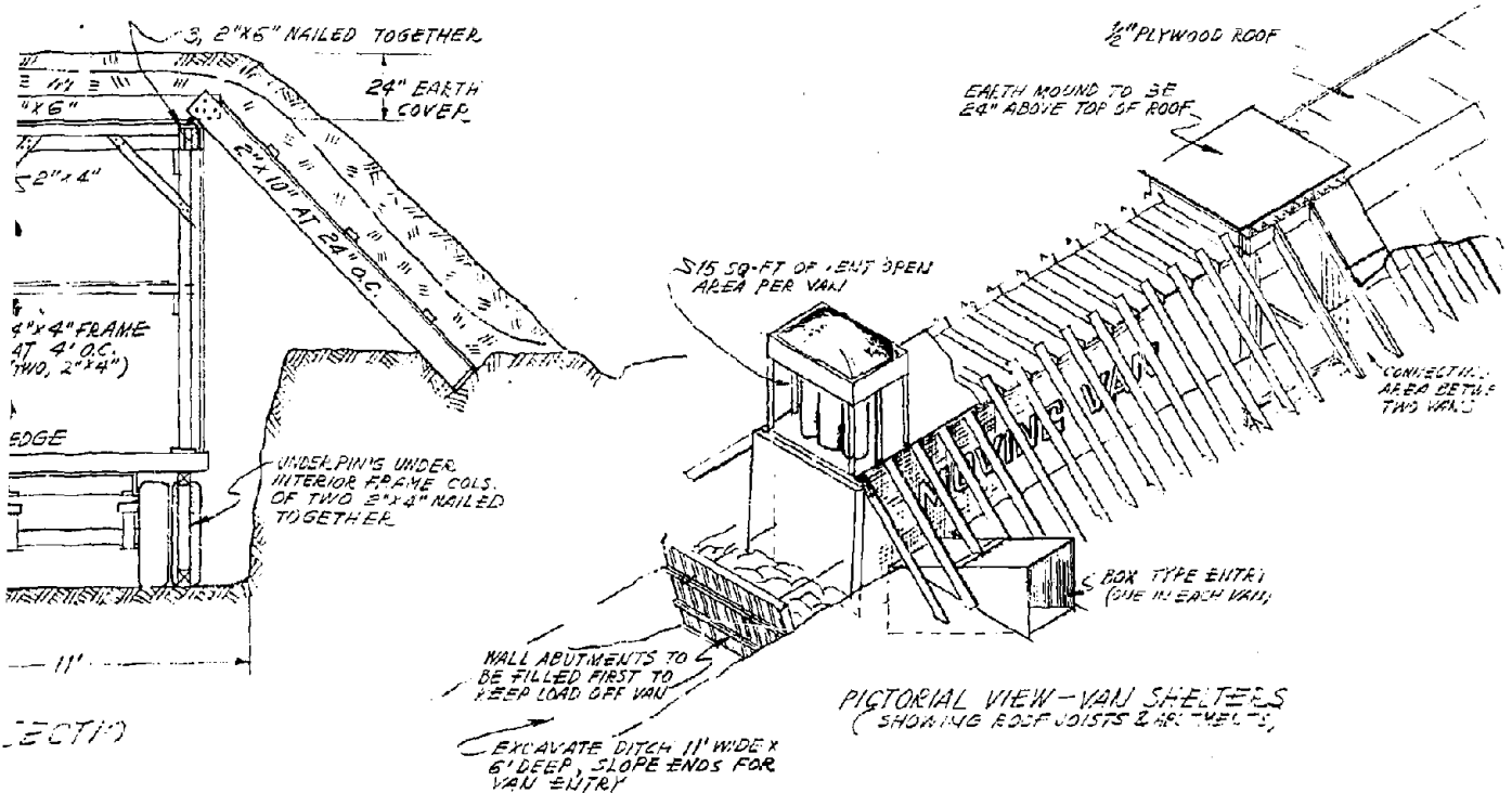
12.1. Trailer Van Shelter, Pictorial View and Sections.
